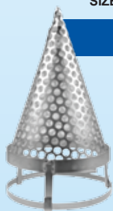
BIRD CONES CONE SS304 FRAME SS201 CLAMP SS201 SIZE 4", 6", 8", 10", 12", 14" & 16"
